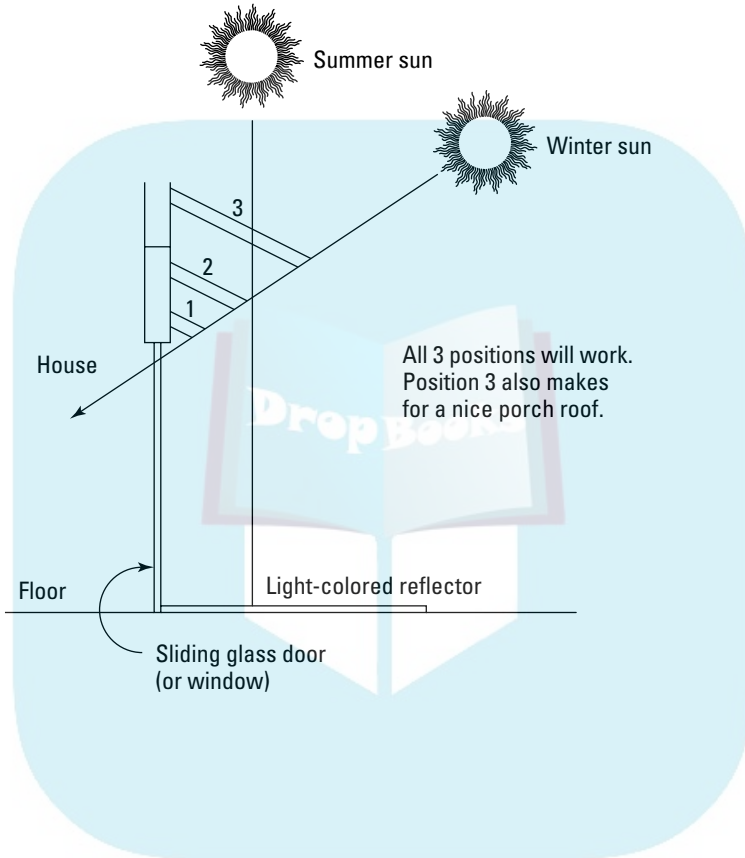
Figure 8-3: Overhangs control sunshine over the seasons.
